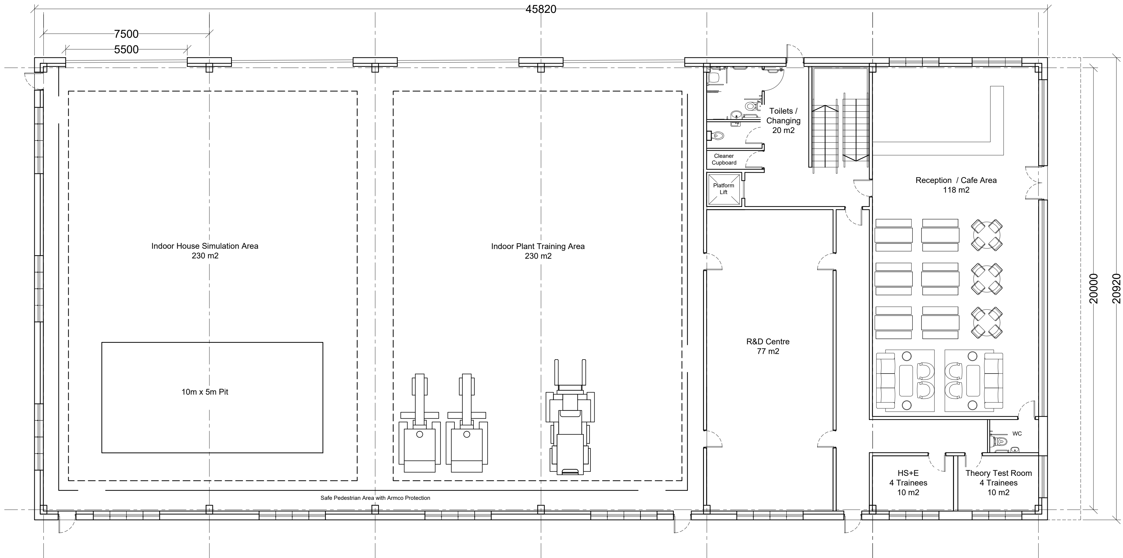
PROPOSED GROUND FLOOR
