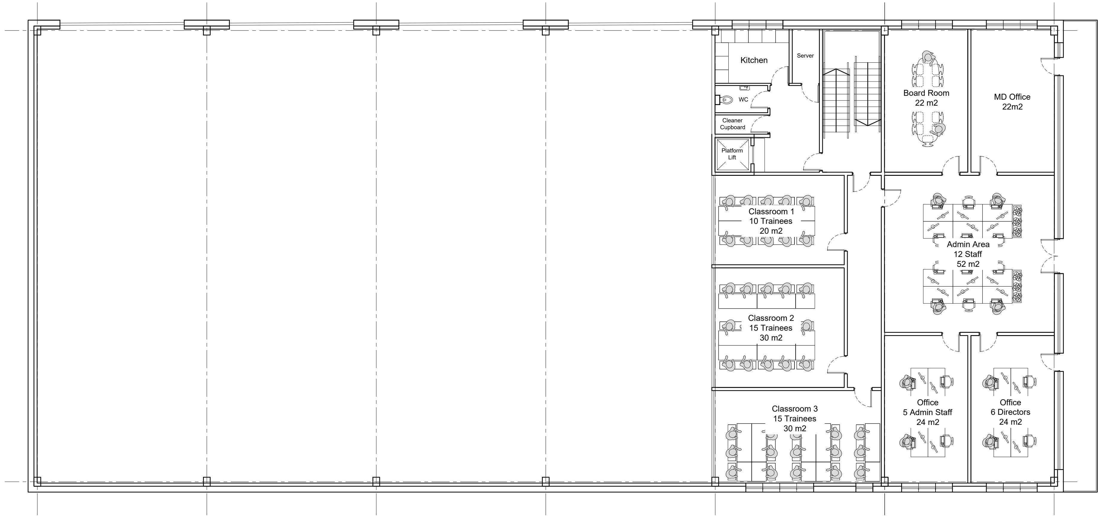
PROPOSED FIRST FLOOR
