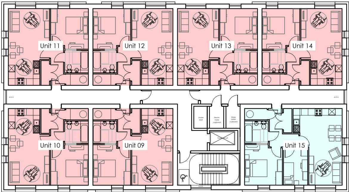
First Floor Plan - 463 m2 GIA
