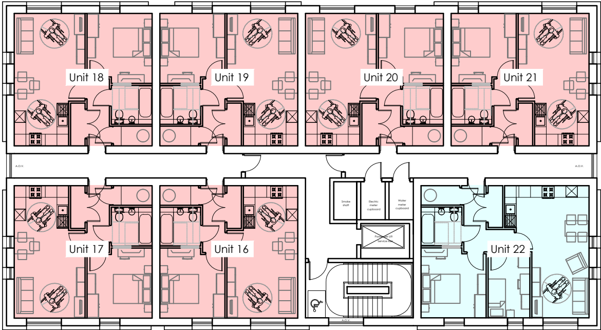
Second Floor Plan - 463 m2 GIA
