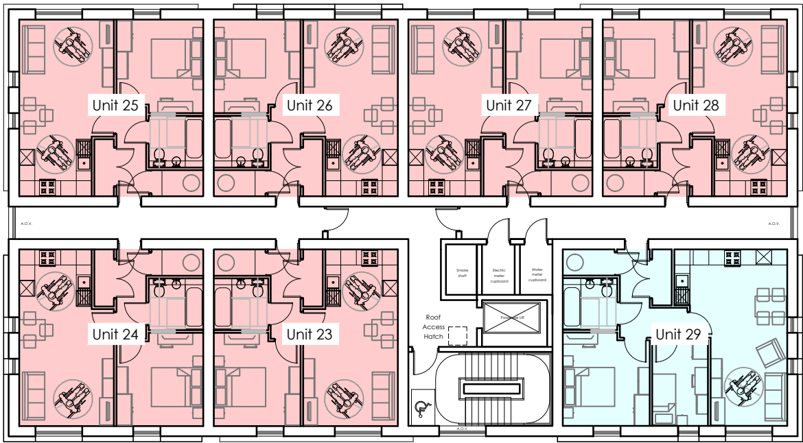
Third Floor Plan - 463 m2 GIA
